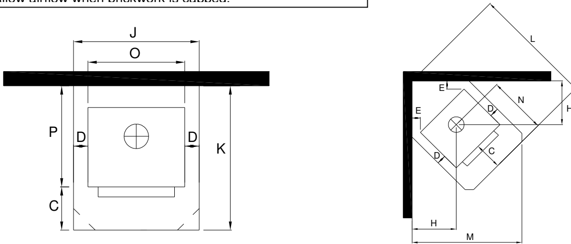
FIG D: MINIMUM FIRE TO COMBUSTABLE WALL CLEARANCES - HOBSON (WITH YUNCA FLUE MOUNTED SHIELD FITTED). Measurements in millimetres.
